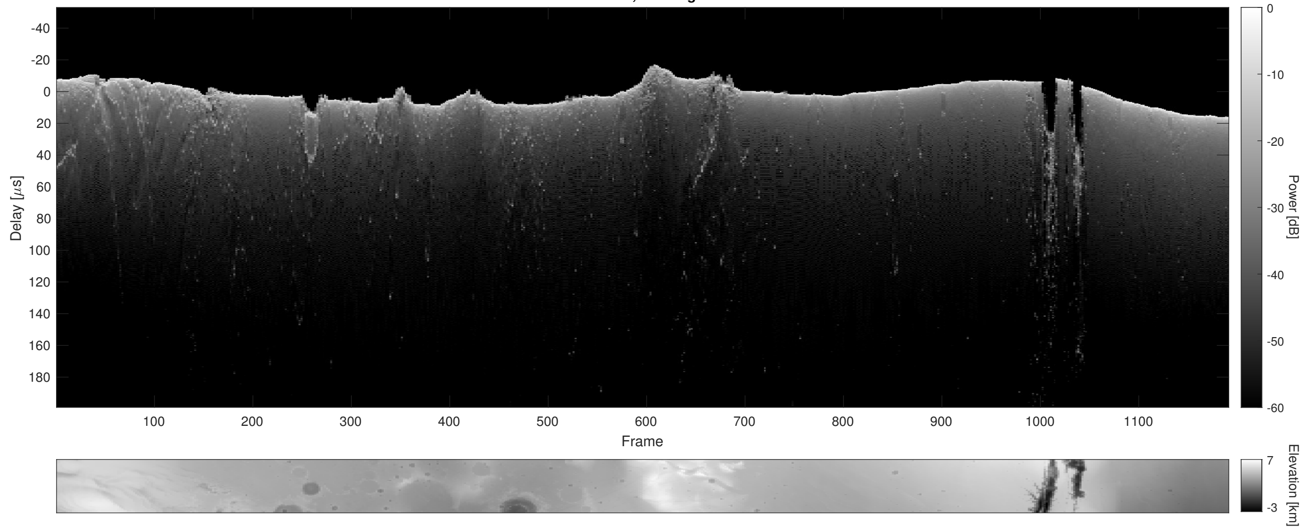
Orbit 8459, Cluttergram
