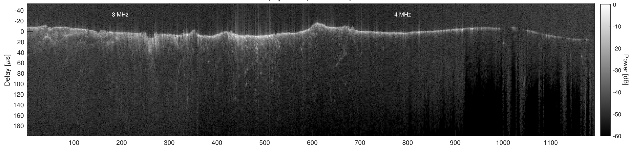
Orbit 8459, Cluttergram
