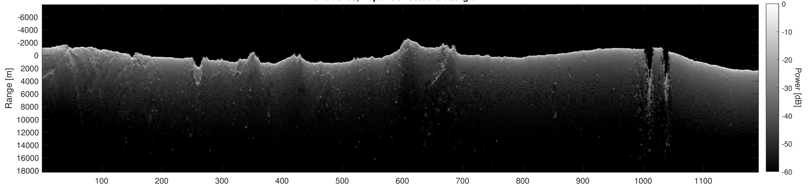
Orbit 8459, Depth-Corrected Cluttergram
