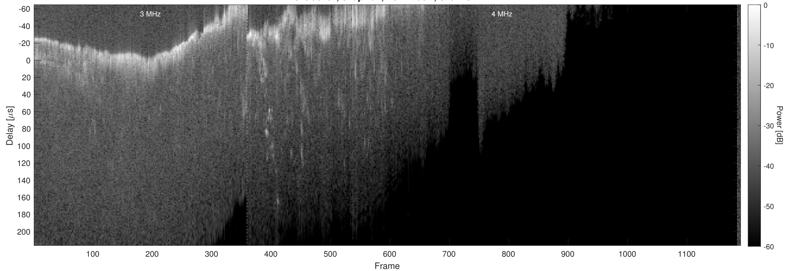
Orbit 8462, Chapman, No Window, Channel 2
