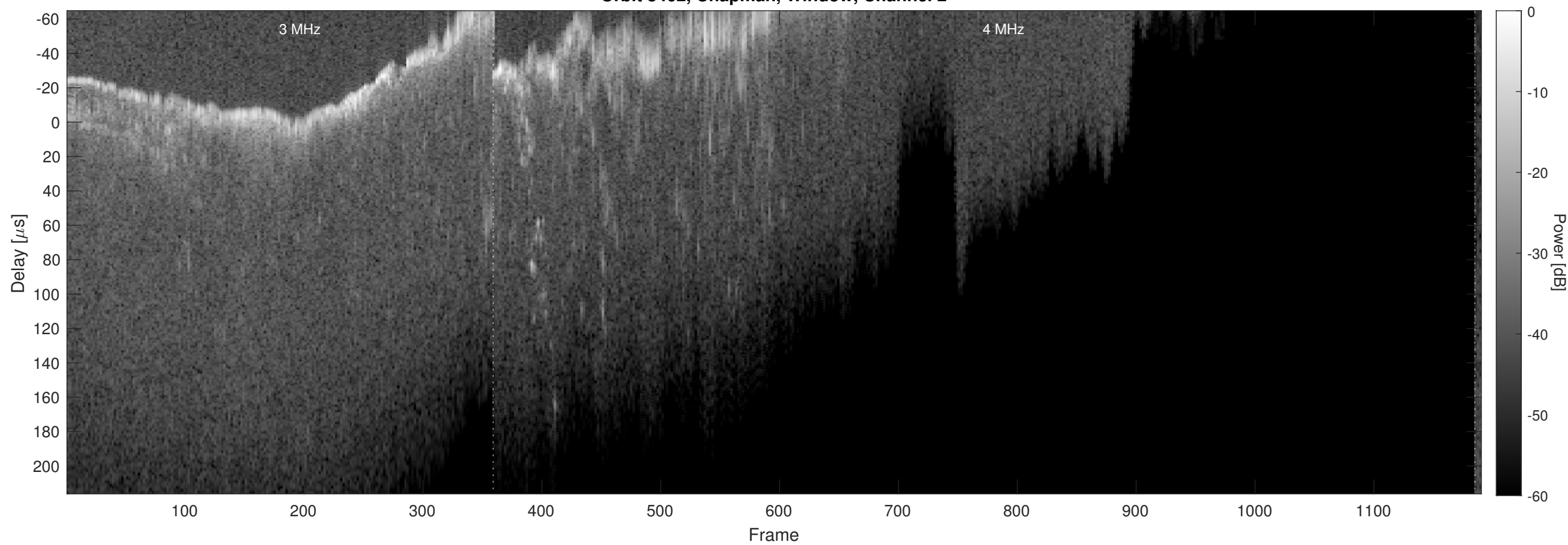
Orbit 8462, Chapman, Window, Channel 2
