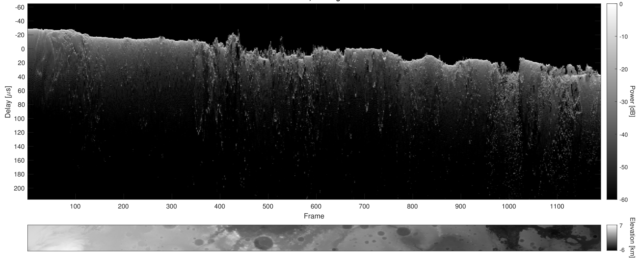
Orbit 8462, Cluttergram
