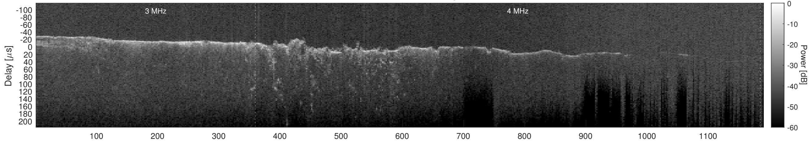
Orbit 8462, Cluttergram
