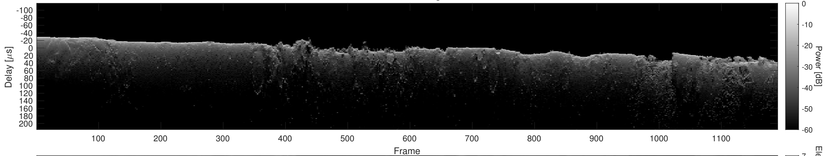
Orbit 8462, Cluttergram
