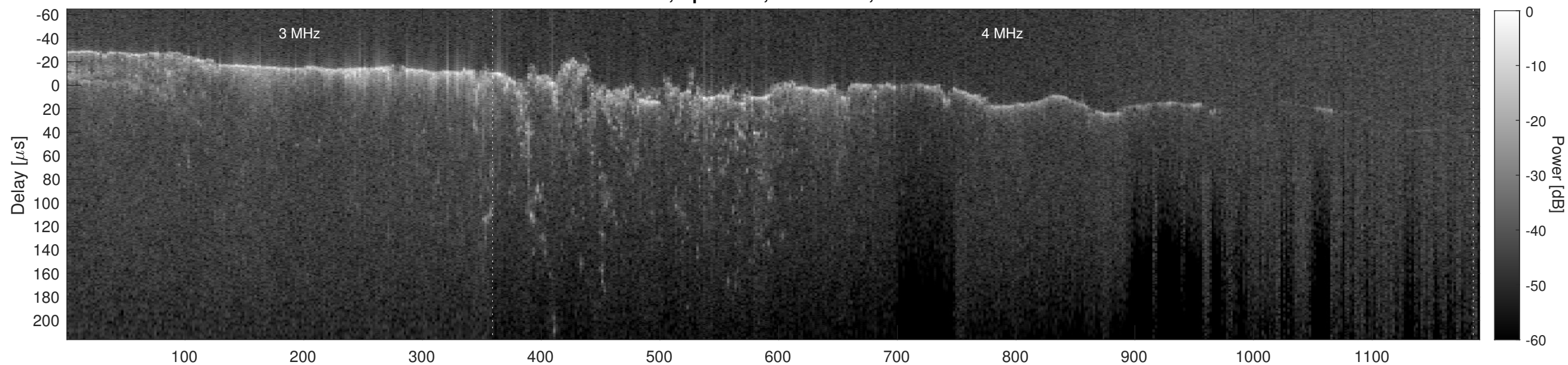
Orbit 8462, Cluttergram
