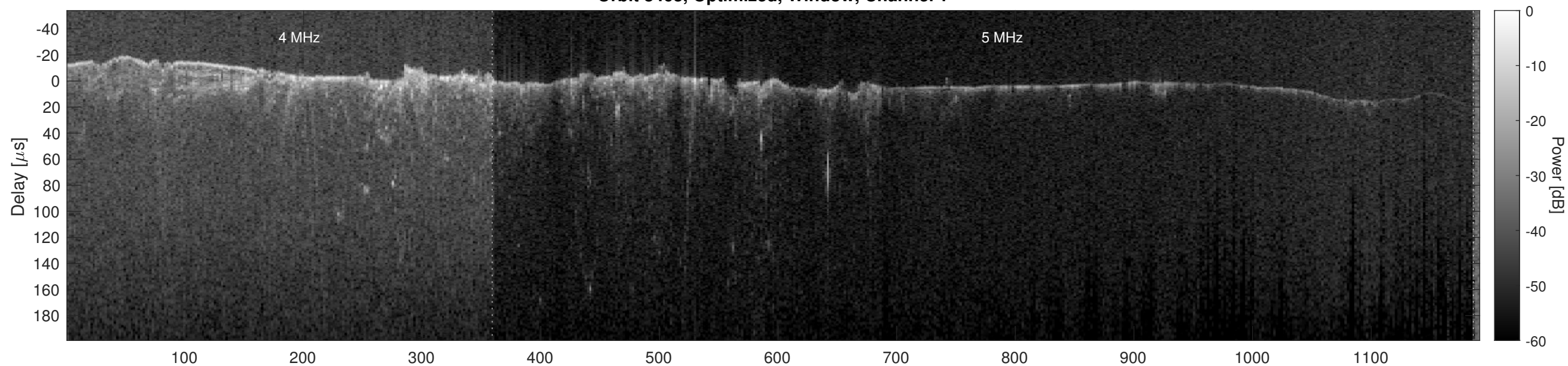
Orbit 8463, Optimized, Window, Channel 2
