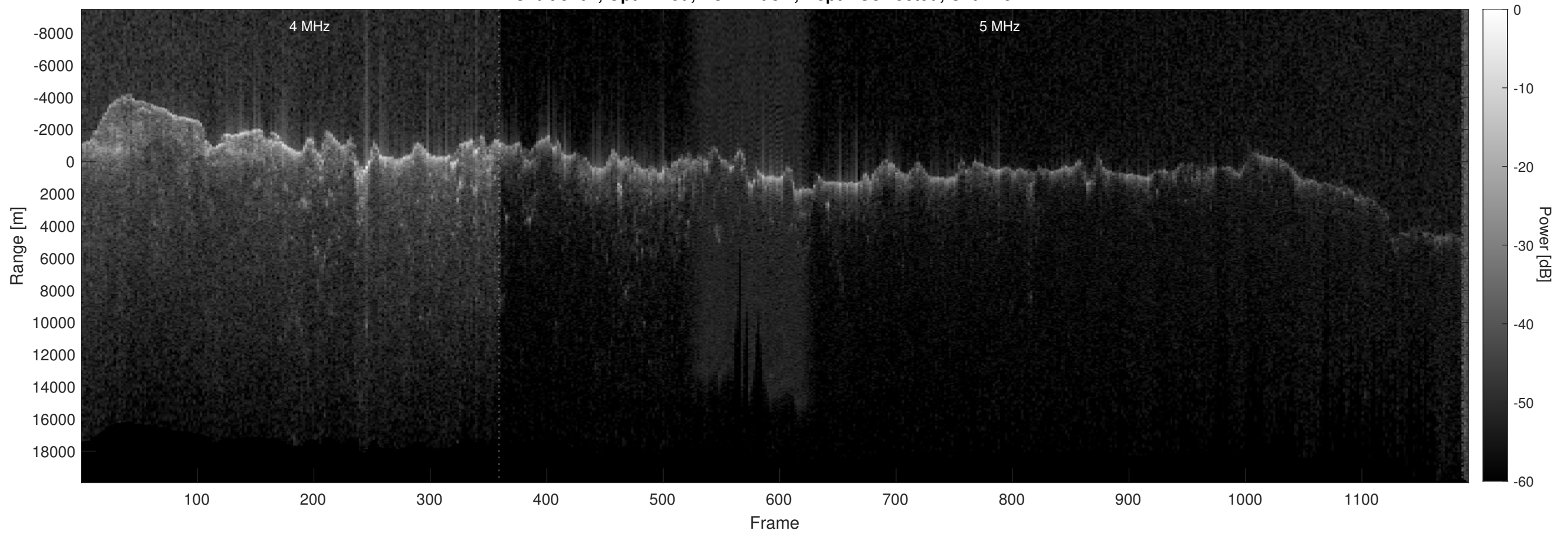
Orbit 8464, Optimized, No Window, Depth-Corrected, Channel 2
