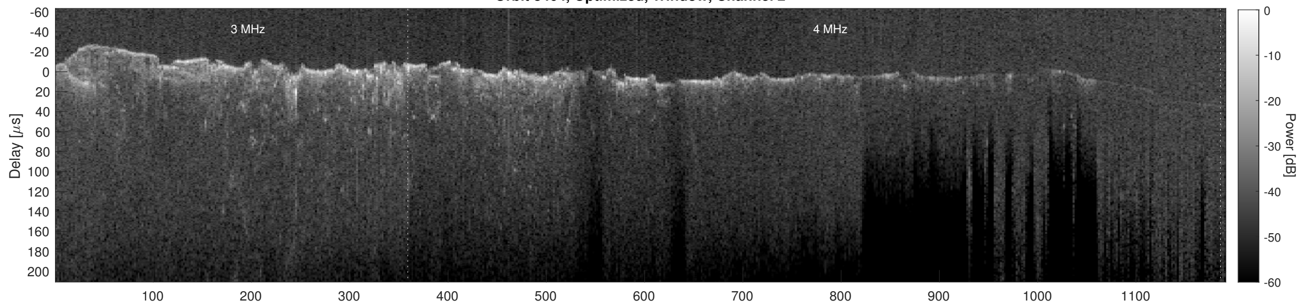
Orbit 8464, Cluttergram
