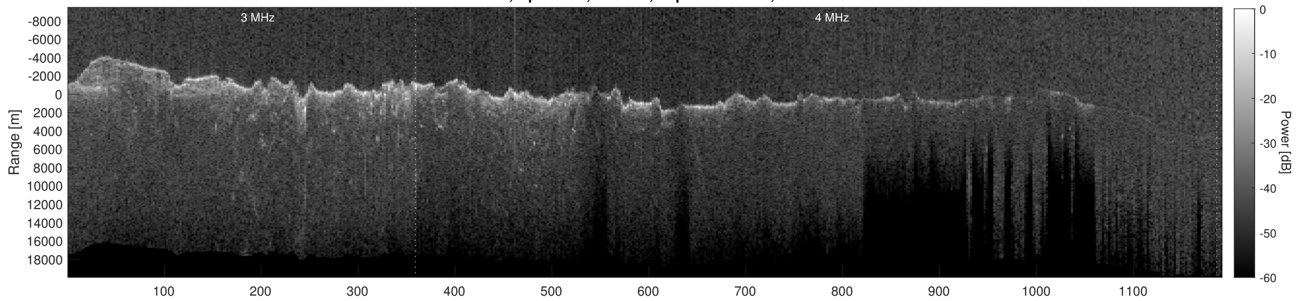
Orbit 8464, Depth-Corrected Cluttergram
