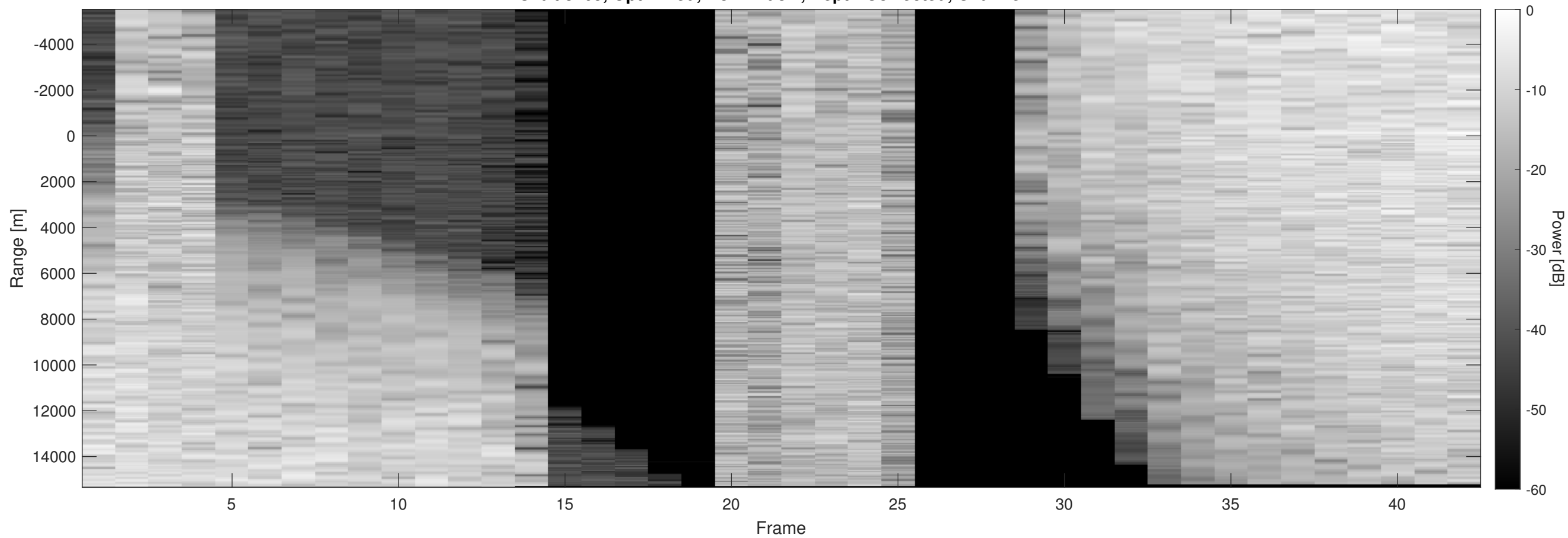
Orbit 8465, Optimized, No Window, Depth-Corrected, Channel 2
