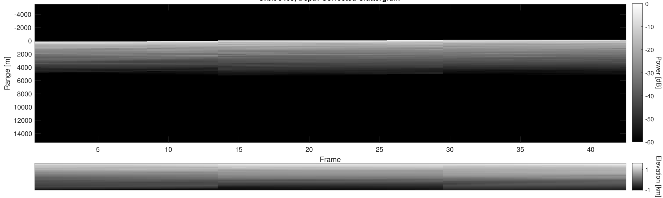
Orbit 8465, Depth-Corrected Cluttergram
