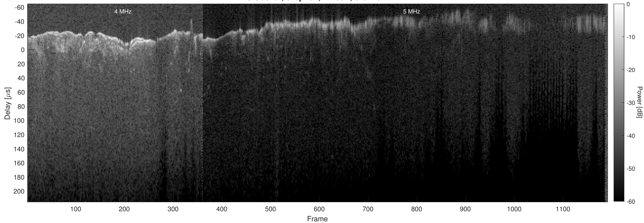
Orbit 8467, Chapman, Window, Channel 2
