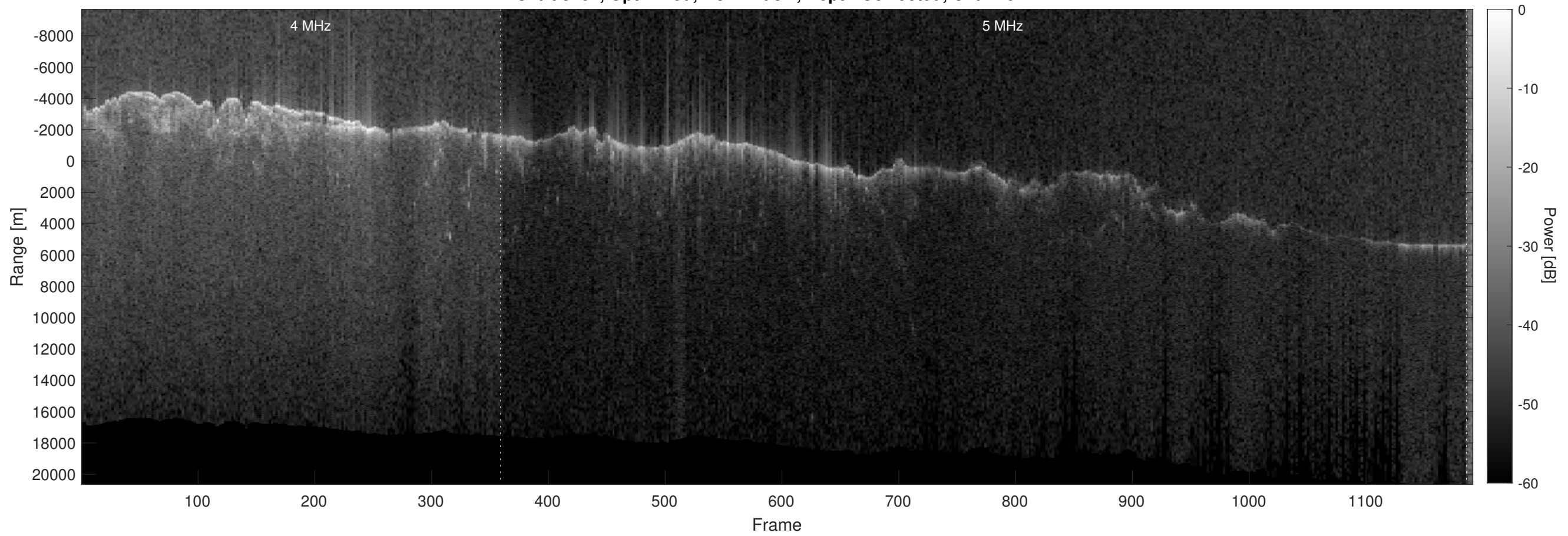
Orbit 8467, Optimized, No Window, Depth-Corrected, Channel 2
