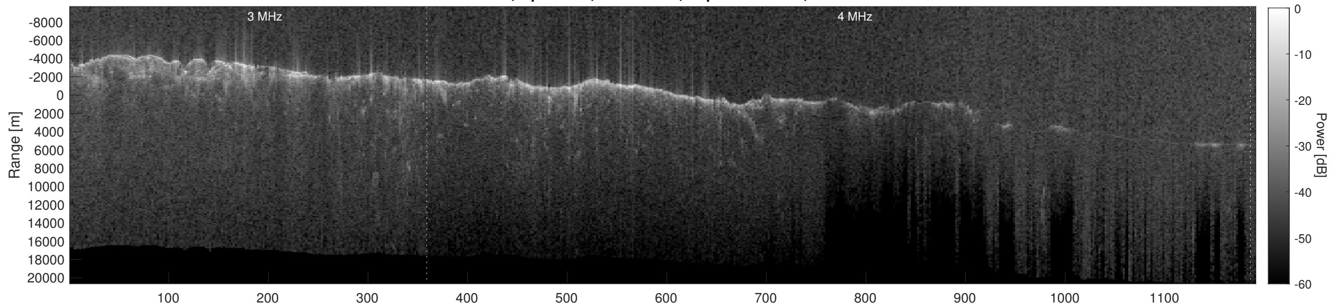
Orbit 8467, Depth-Corrected Cluttergram
