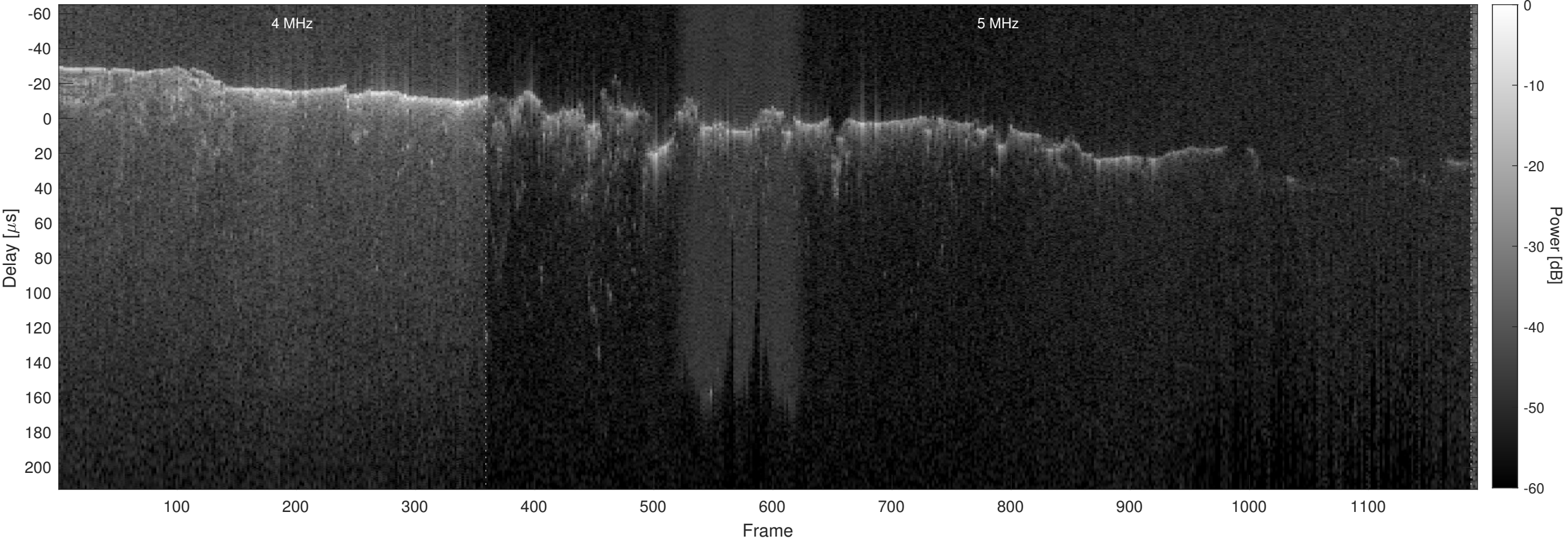
Orbit 8469, Optimized, No Window, Channel 2
