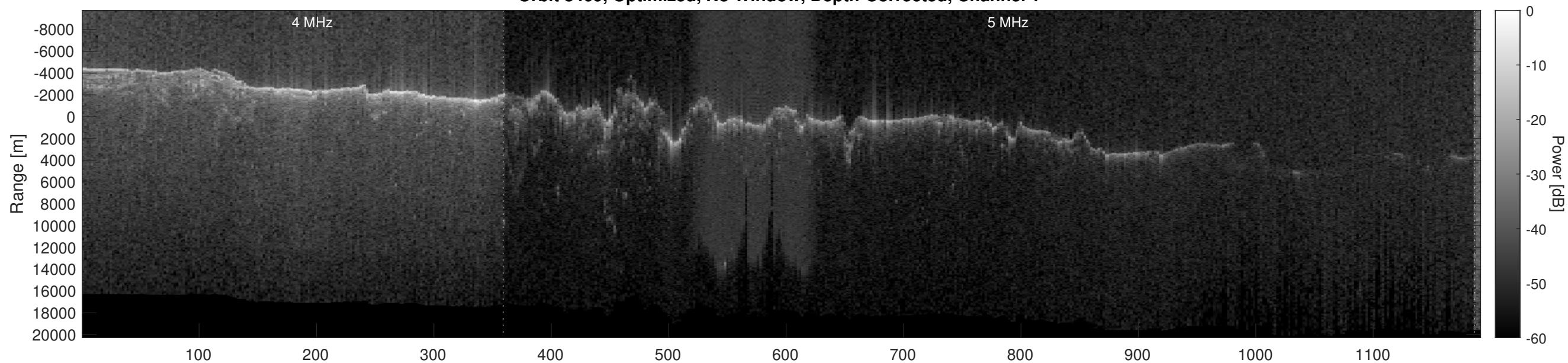
Orbit 8469, Optimized, No Window, Depth-Corrected, Channel 2
