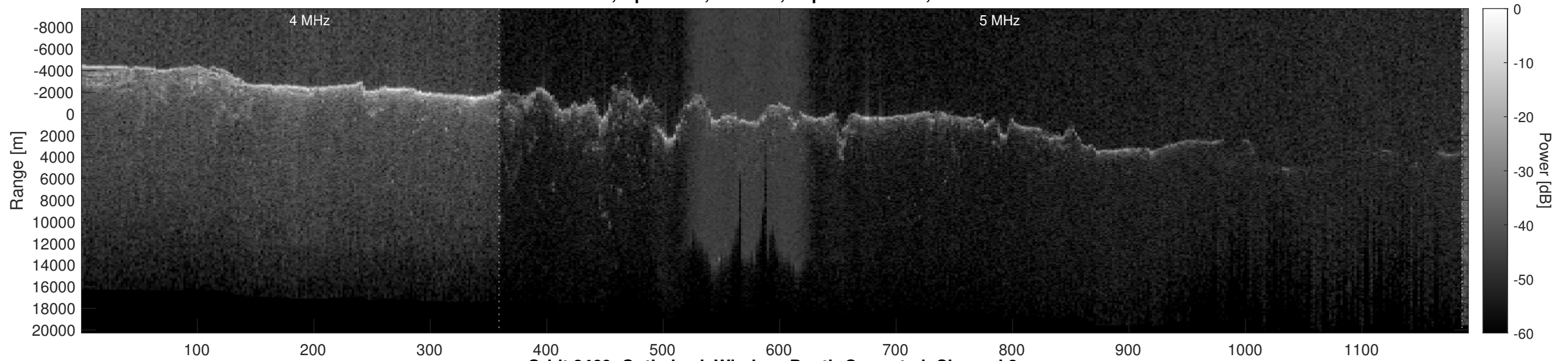
Orbit 8469, Optimized, Window, Depth-Corrected, Channel 2
