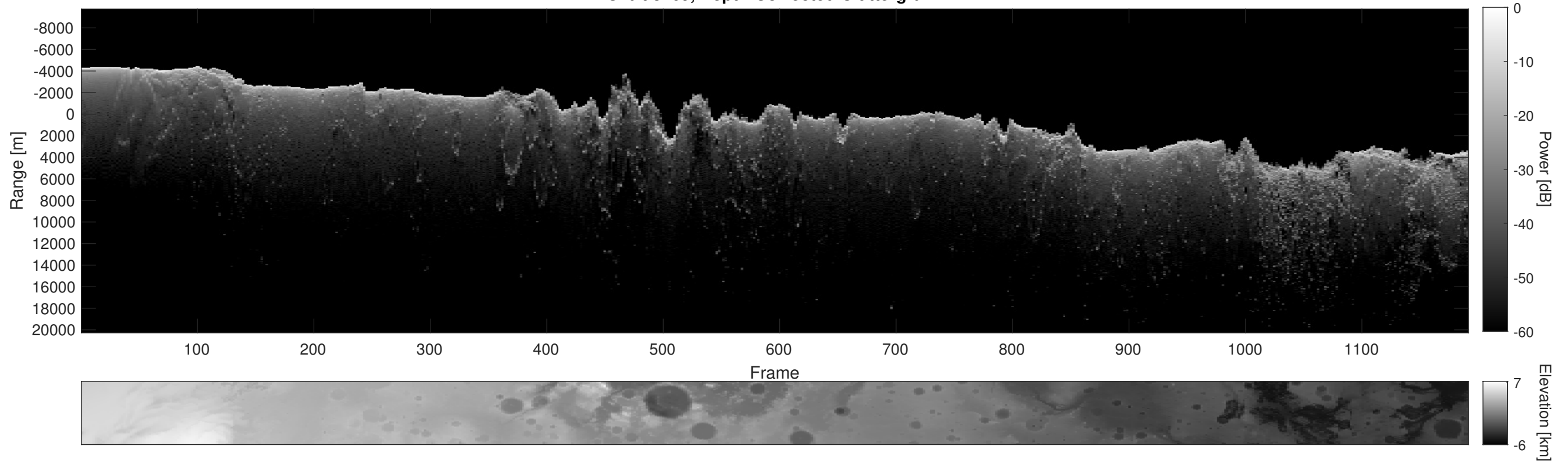
Orbit 8469, Depth-Corrected Cluttergram
