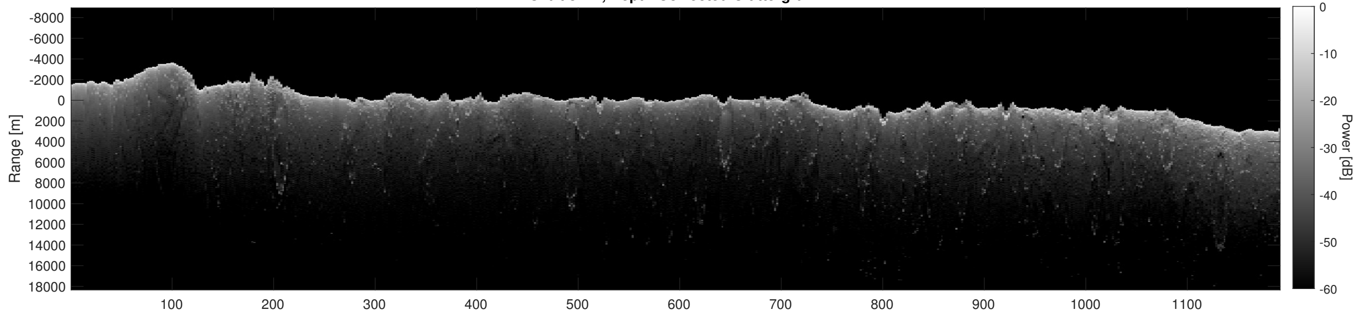
Orbit 8472, Depth-Corrected Cluttergram
