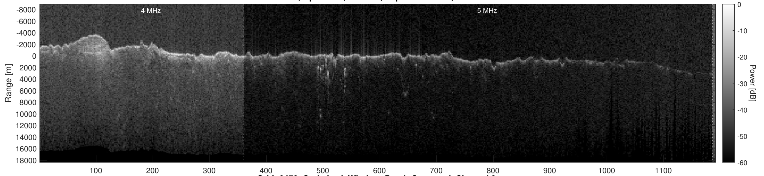
Orbit 8472, Optimized, Window, Depth-Corrected, Channel 2
