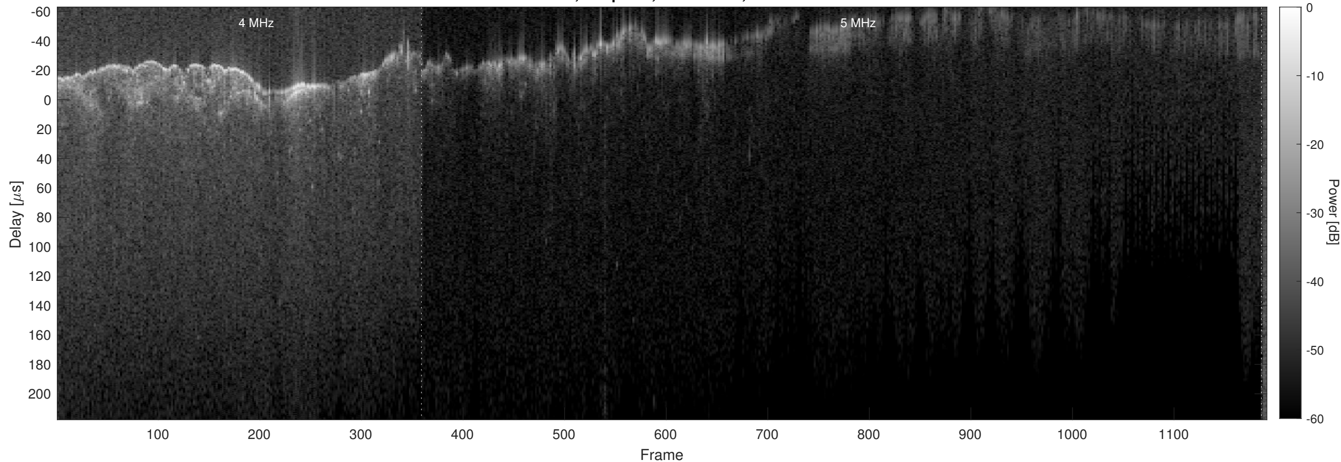
Orbit 8474, Chapman, No Window, Channel 2
