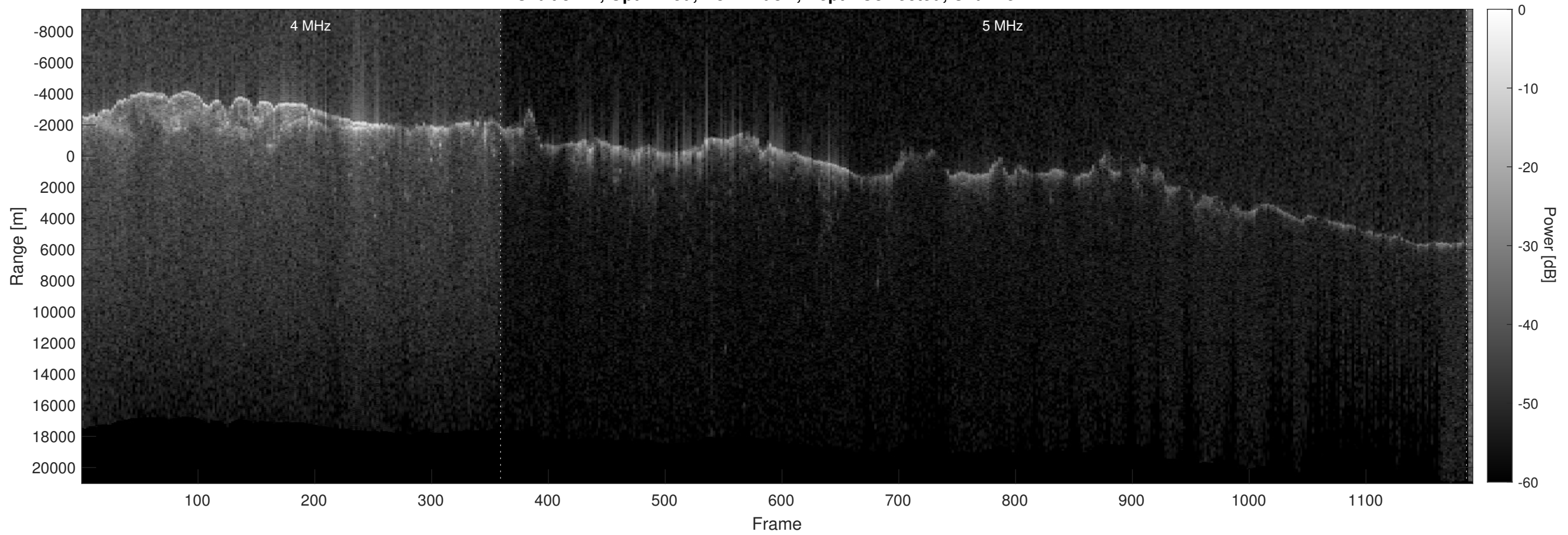
Orbit 8474, Optimized, No Window, Depth-Corrected, Channel 2
