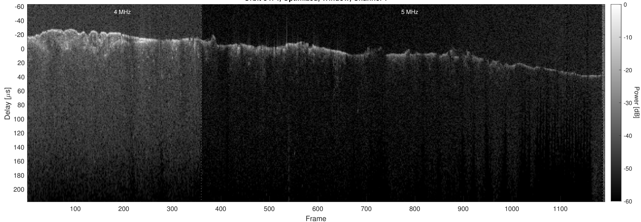
Orbit 8474, Optimized, Window, Channel 2
