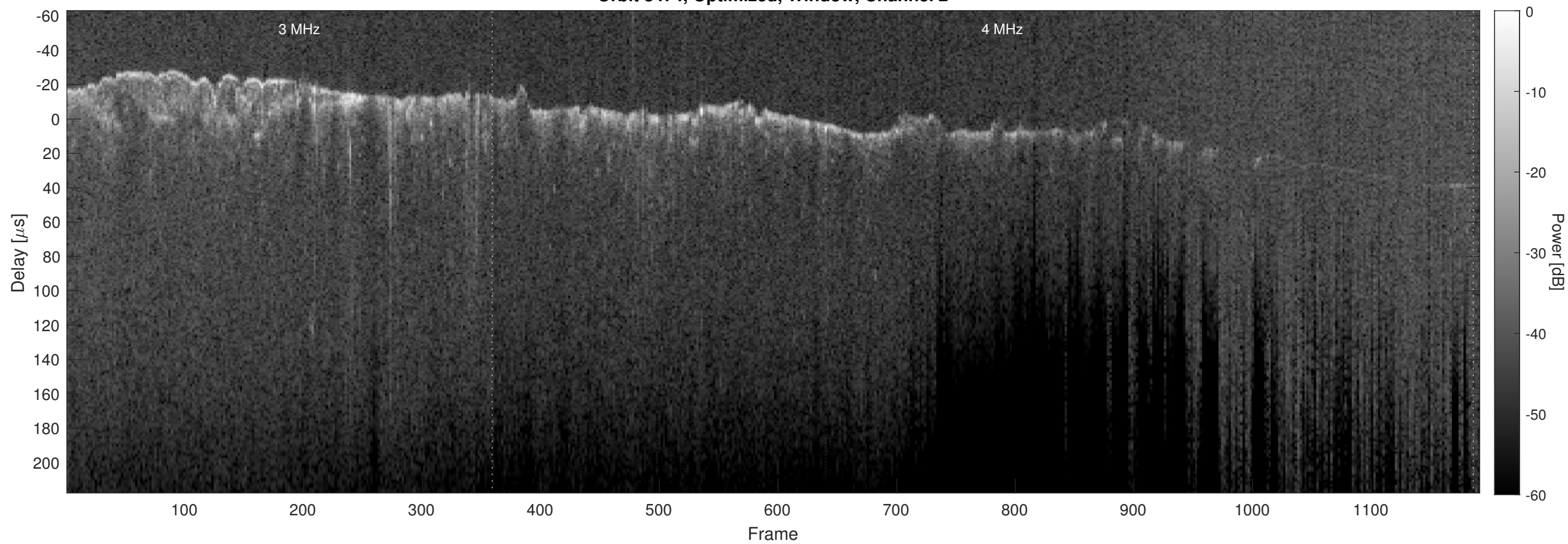
Orbit 8474, Optimized, Window, Channel 2
