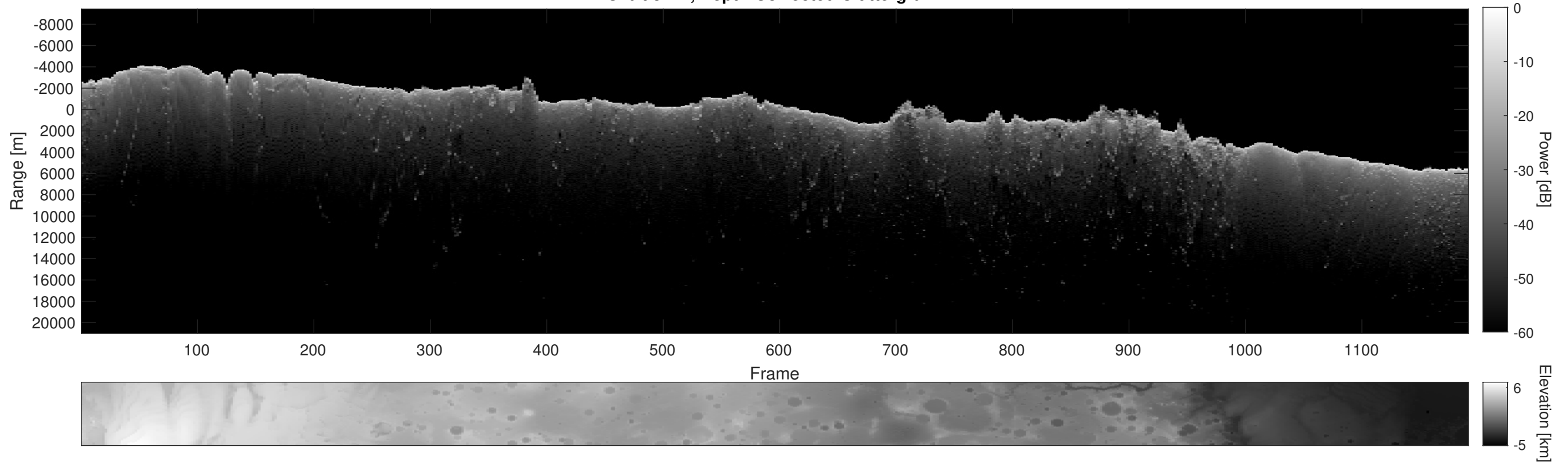
Orbit 8474, Depth-Corrected Cluttergram
