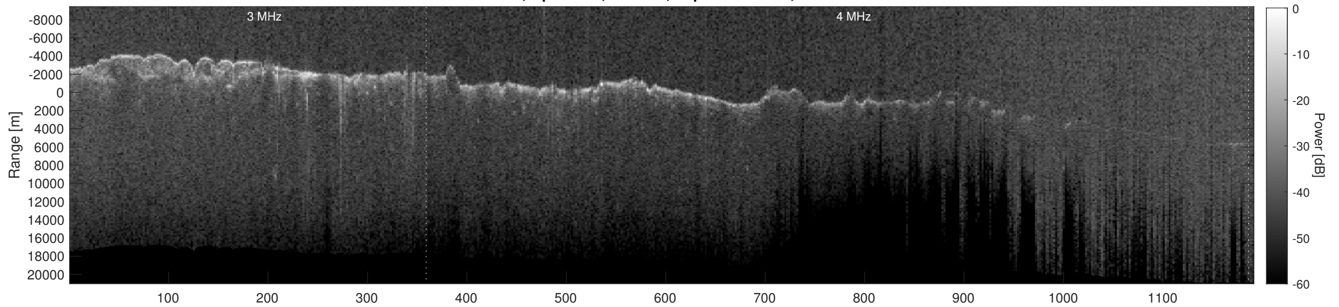
Orbit 8474, Depth-Corrected Cluttergram
