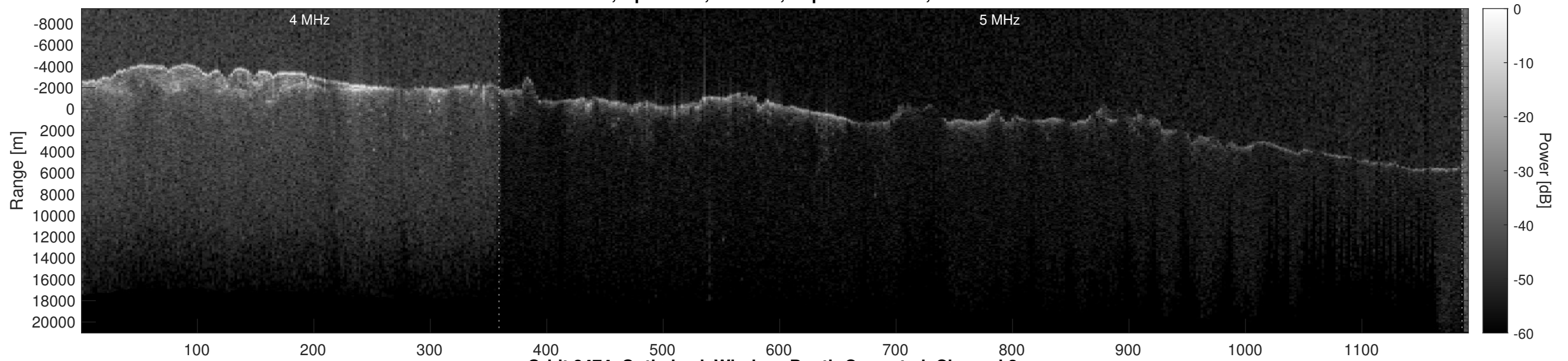
Orbit 8474, Optimized, Window, Depth-Corrected, Channel 2
