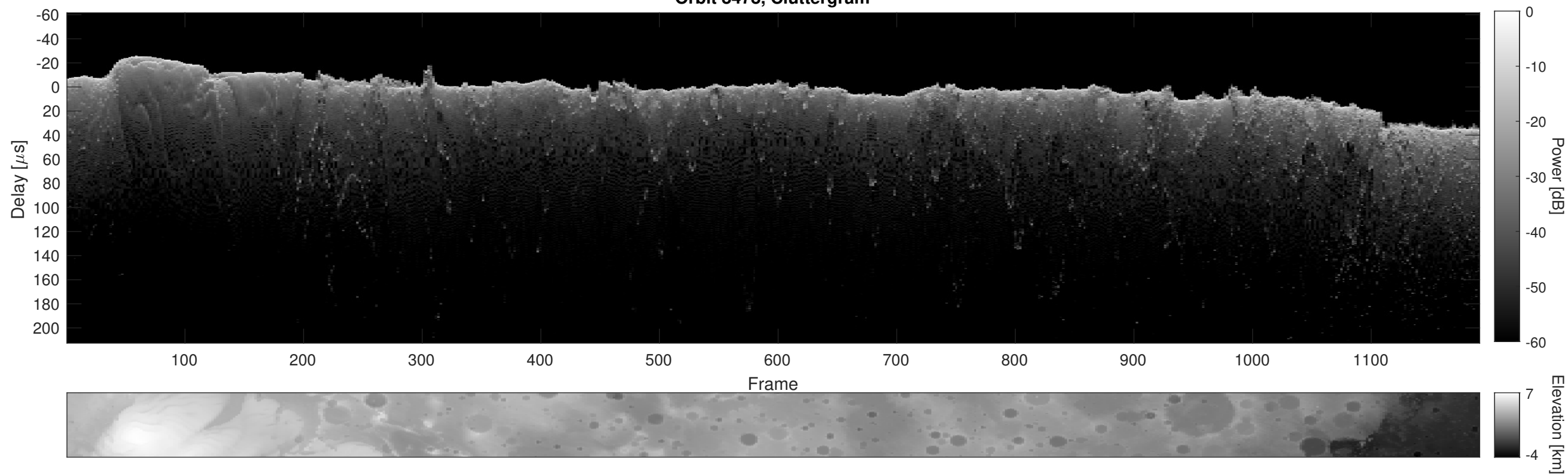
Orbit 8478, Cluttergram
