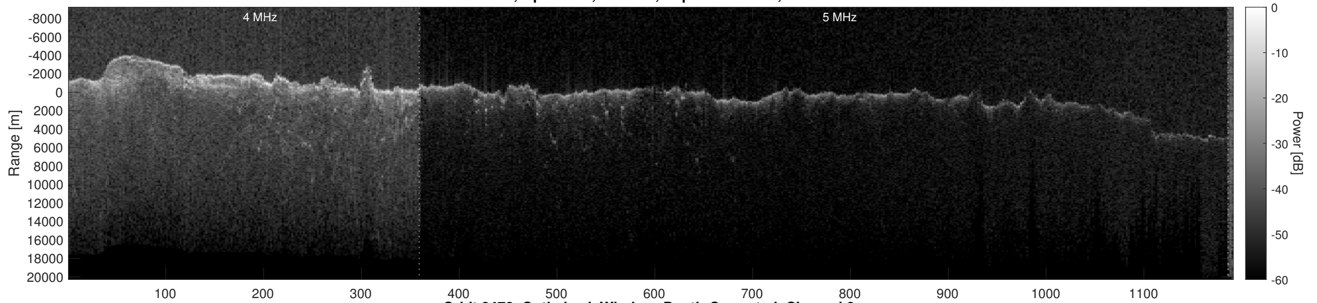
Orbit 8478, Optimized, Window, Depth-Corrected, Channel 2
