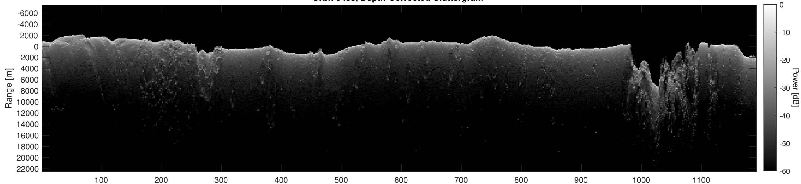
Orbit 8480, Depth-Corrected Cluttergram
