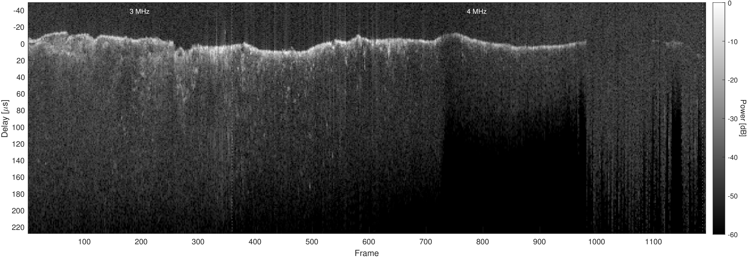
Orbit 8480, Optimized, Window, Channel 2
