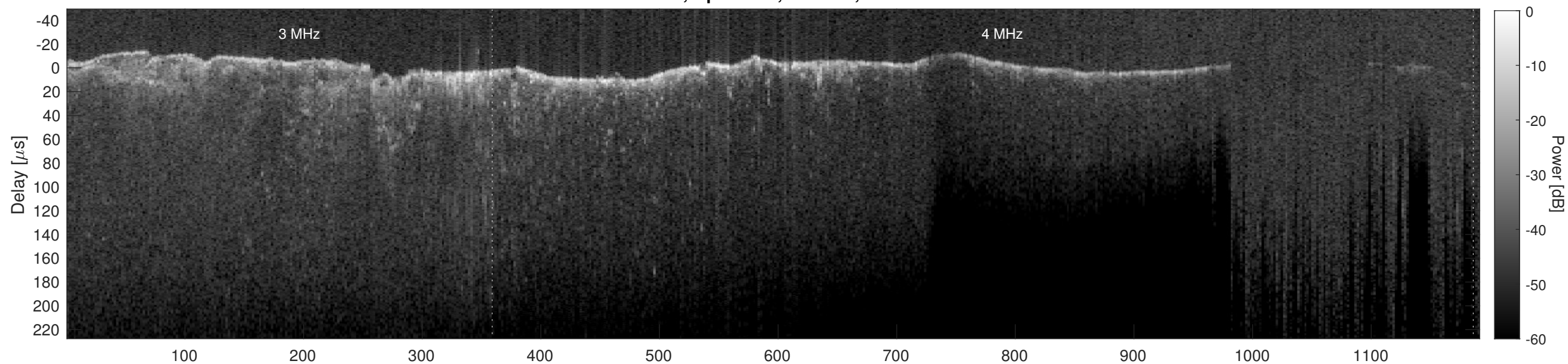
Orbit 8480, Cluttergram
