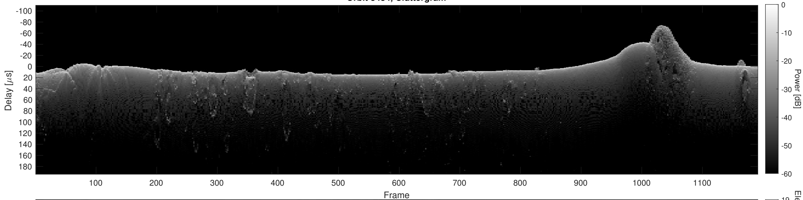
Orbit 8484, Cluttergram
