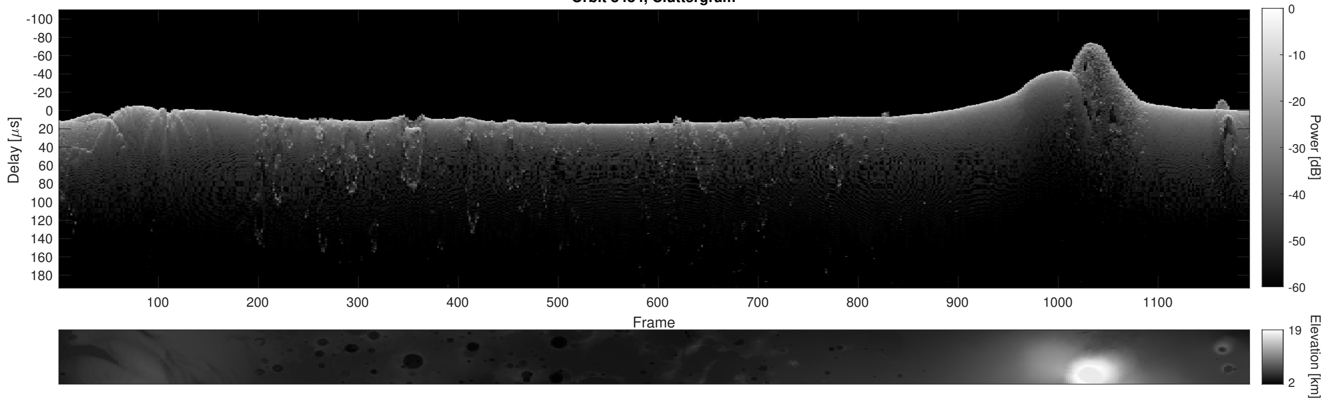
Orbit 8484, Cluttergram
