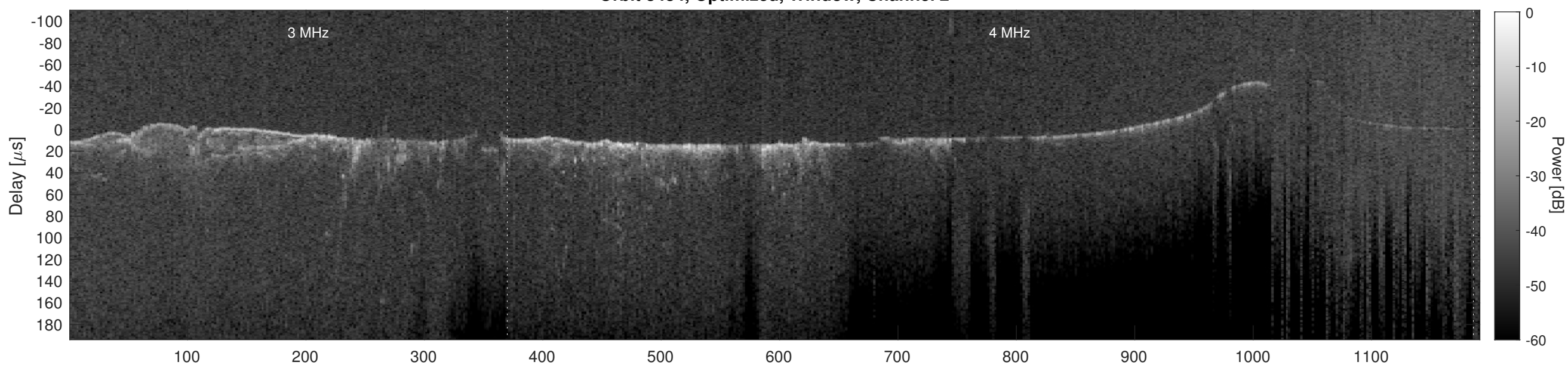
Orbit 8484, Cluttergram
