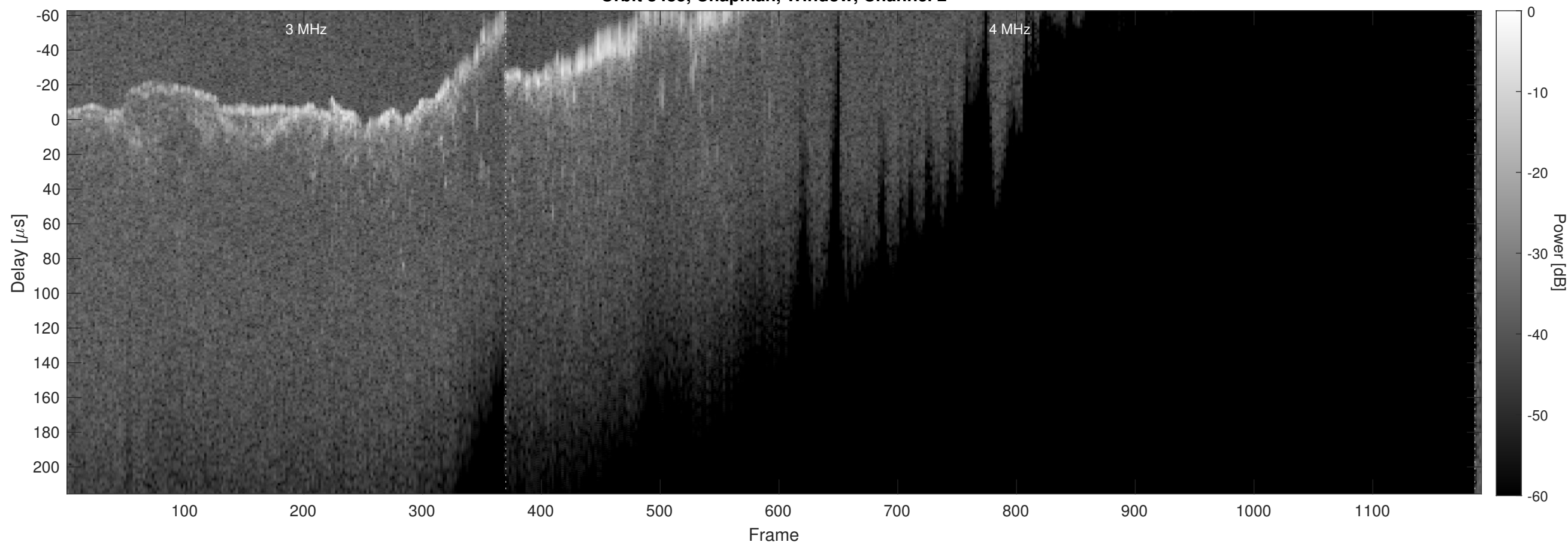
Orbit 8485, Chapman, Window, Channel 2
