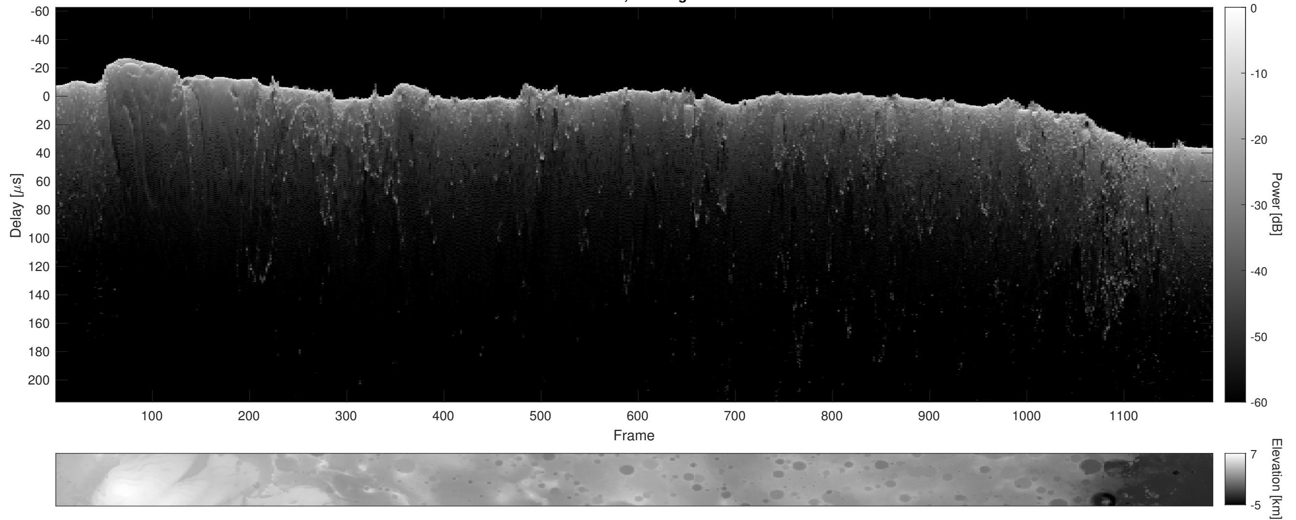
Orbit 8485, Cluttergram
