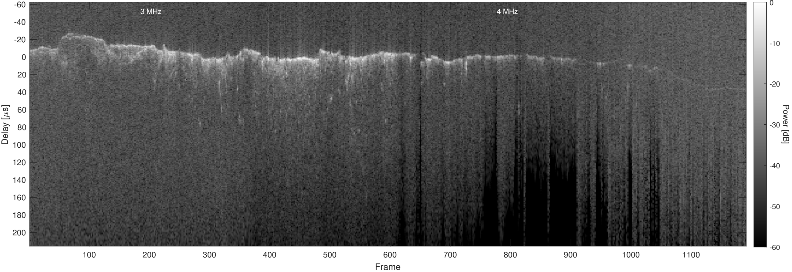
Orbit 8485, Optimized, No Window, Channel 2
