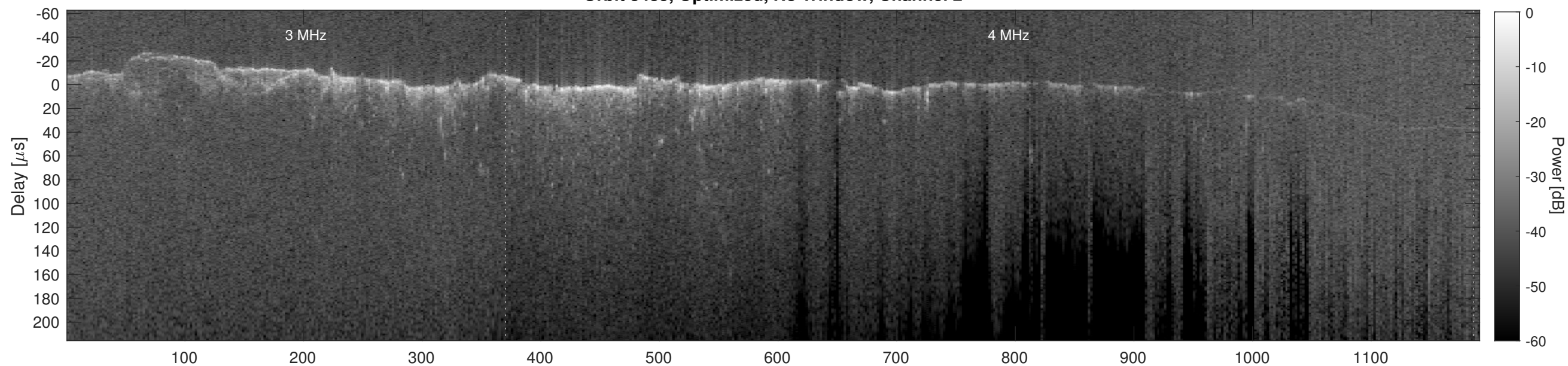
Orbit 8485, Cluttergram
