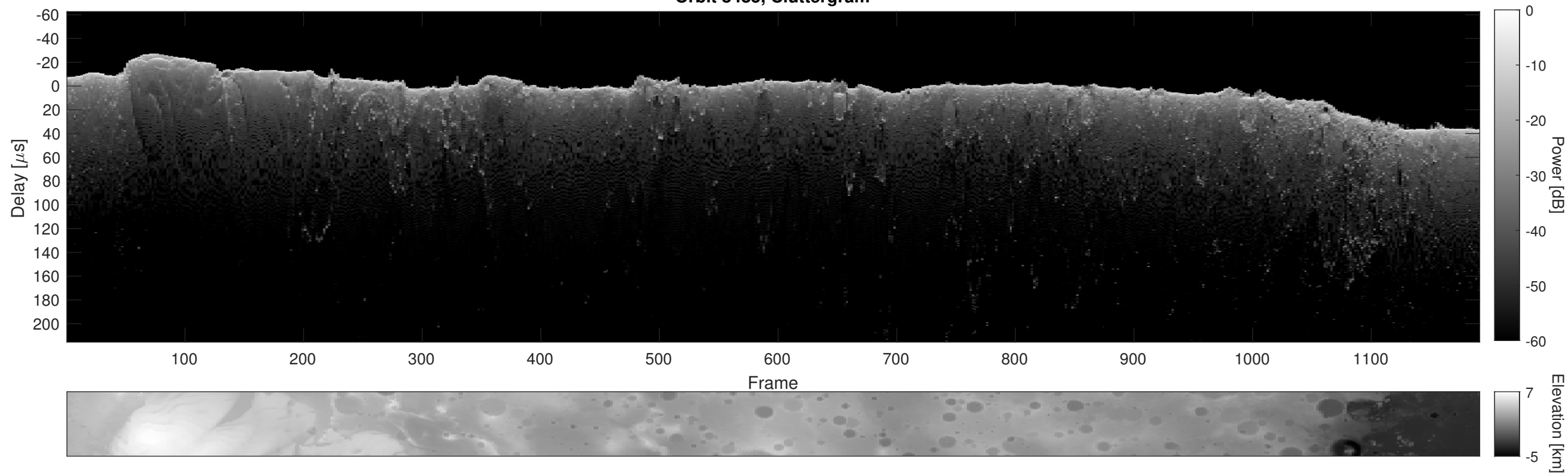
Orbit 8485, Cluttergram
