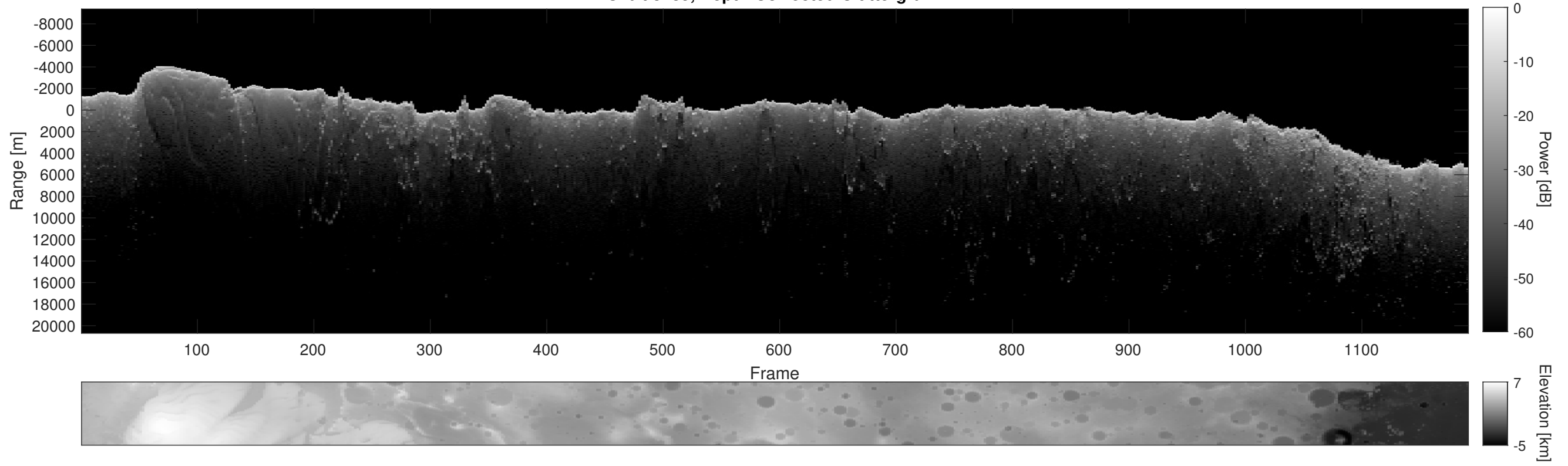
Orbit 8485, Depth-Corrected Cluttergram
