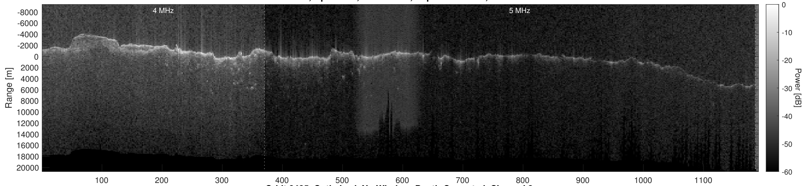
Orbit 8485, Optimized, No Window, Depth-Corrected, Channel 2
