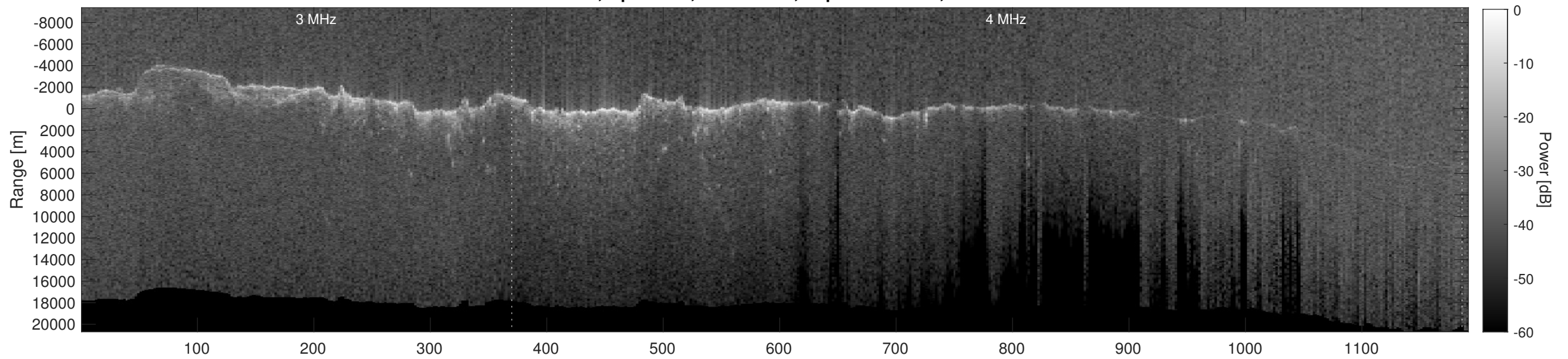
Orbit 8485, Depth-Corrected Cluttergram
