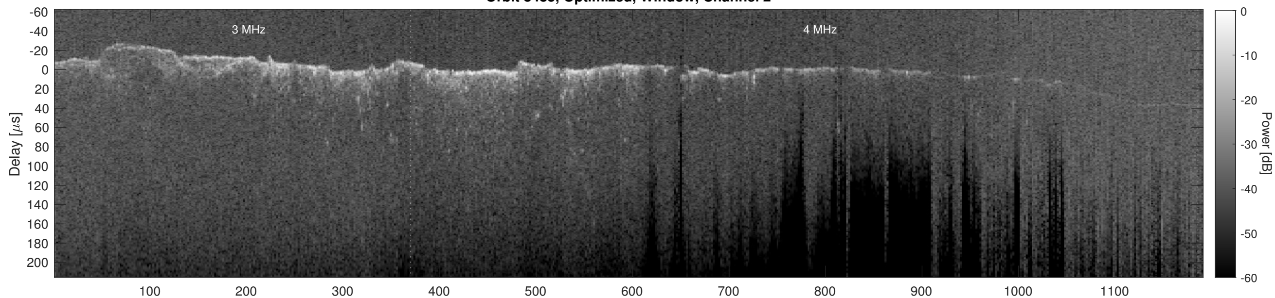
Orbit 8485, Cluttergram
