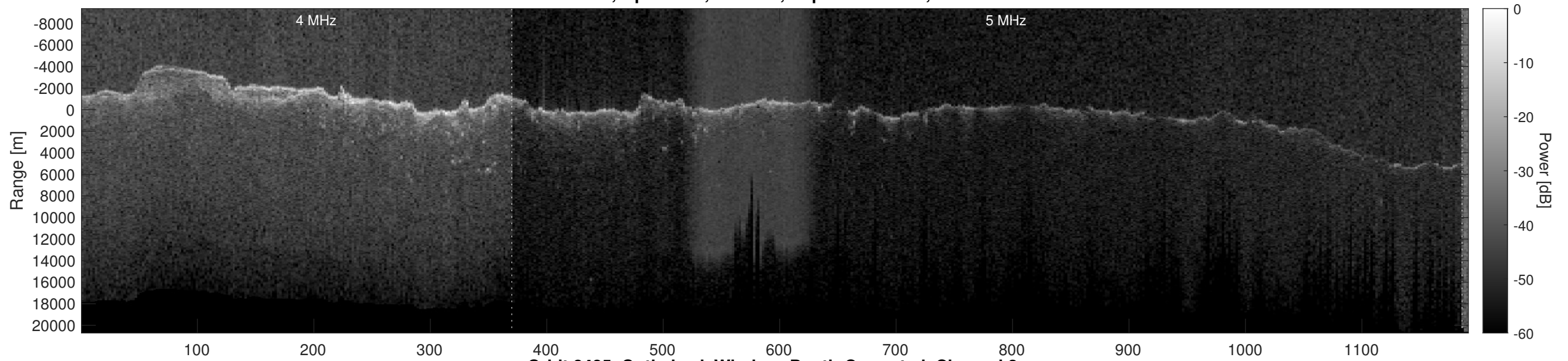
Orbit 8485, Optimized, Window, Depth-Corrected, Channel 2
