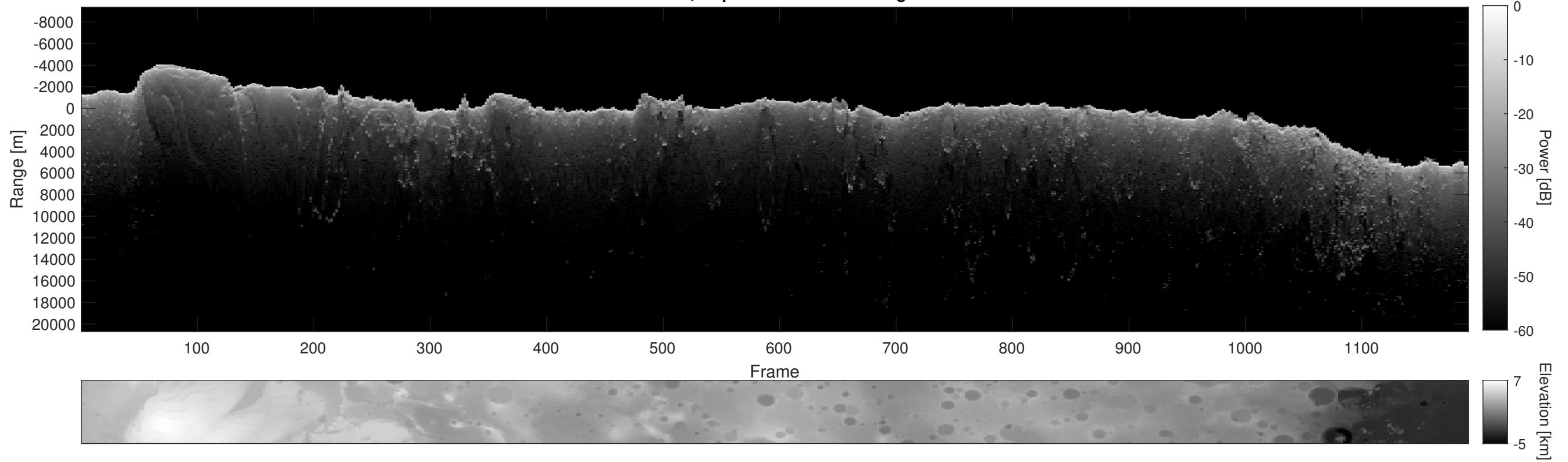
Orbit 8485, Depth-Corrected Cluttergram
