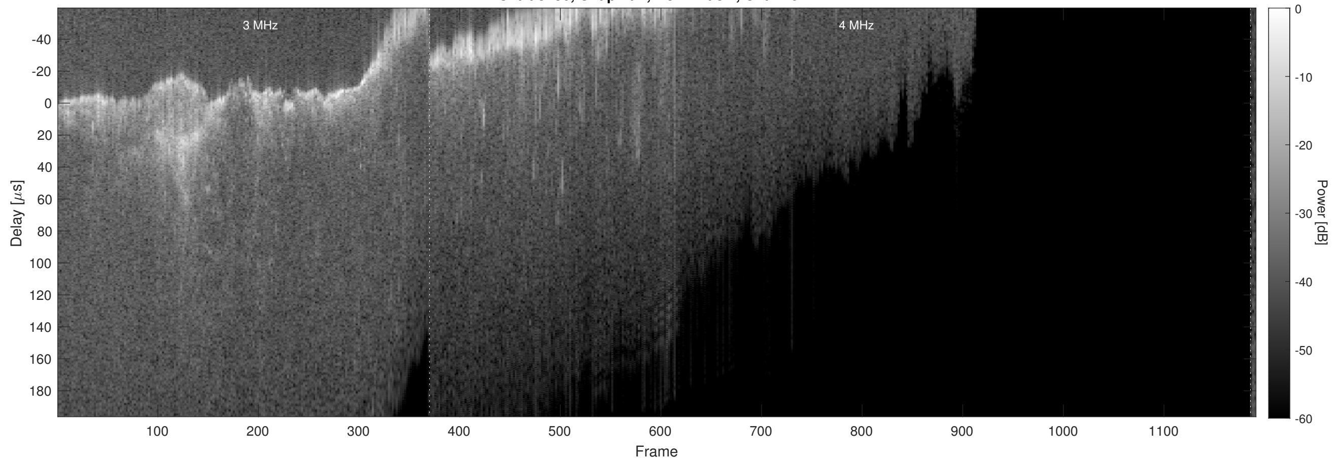
Orbit 8486, Chapman, No Window, Channel 2
