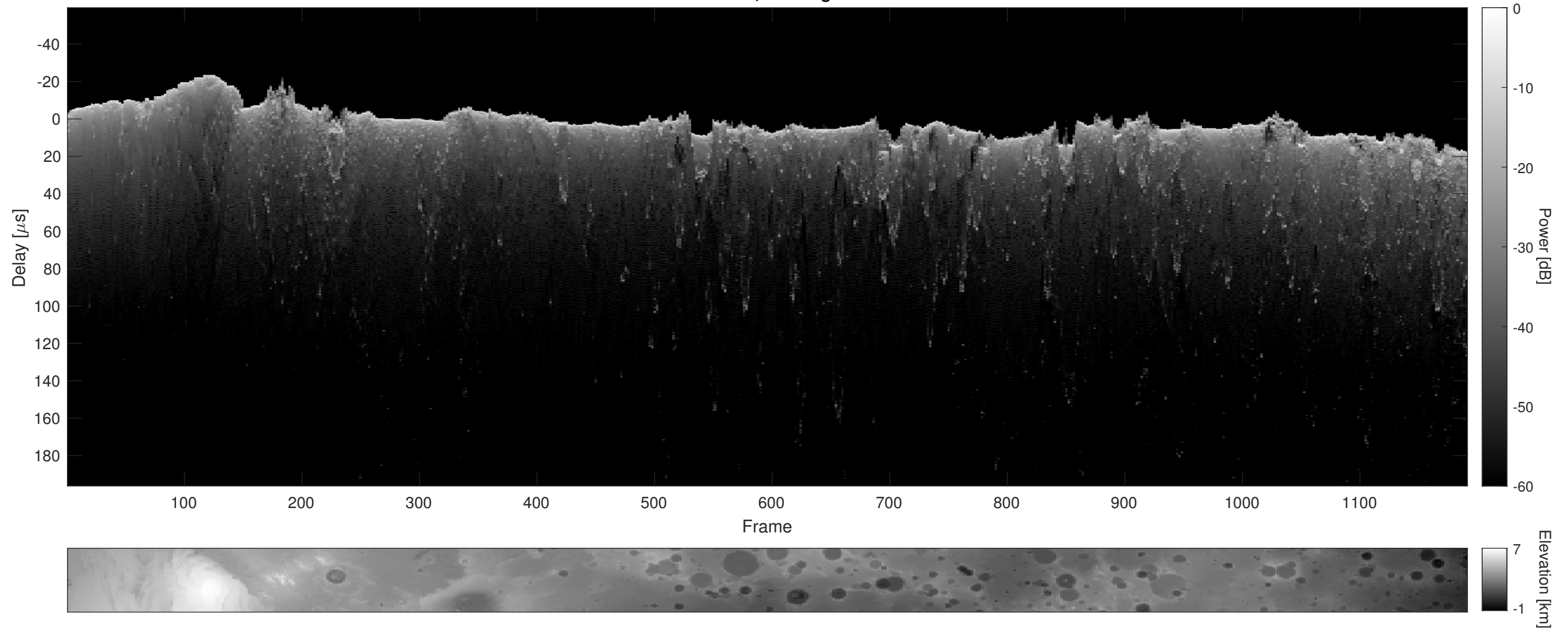
Orbit 8486, Cluttergram
