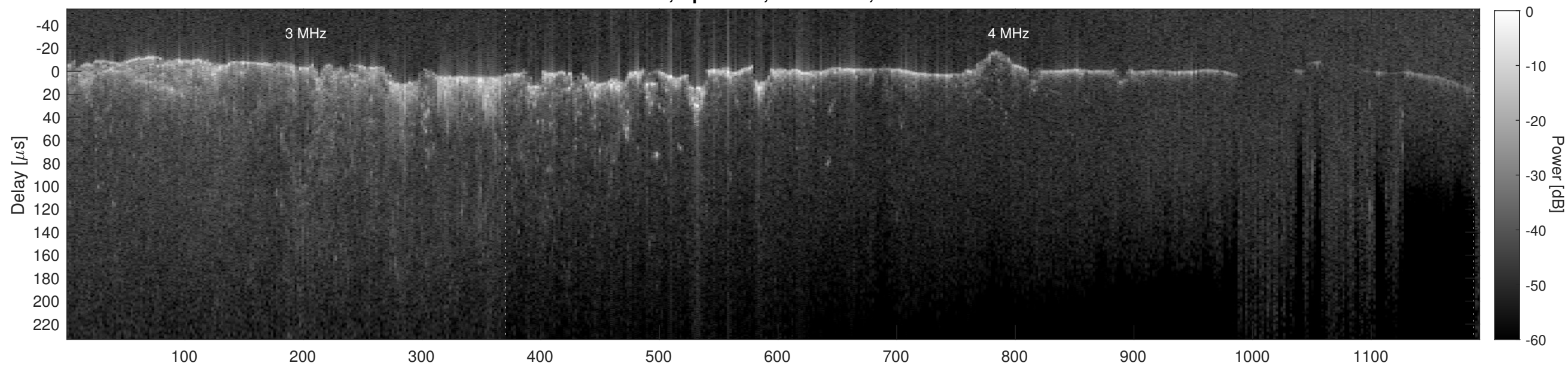
Orbit 8487, Cluttergram
