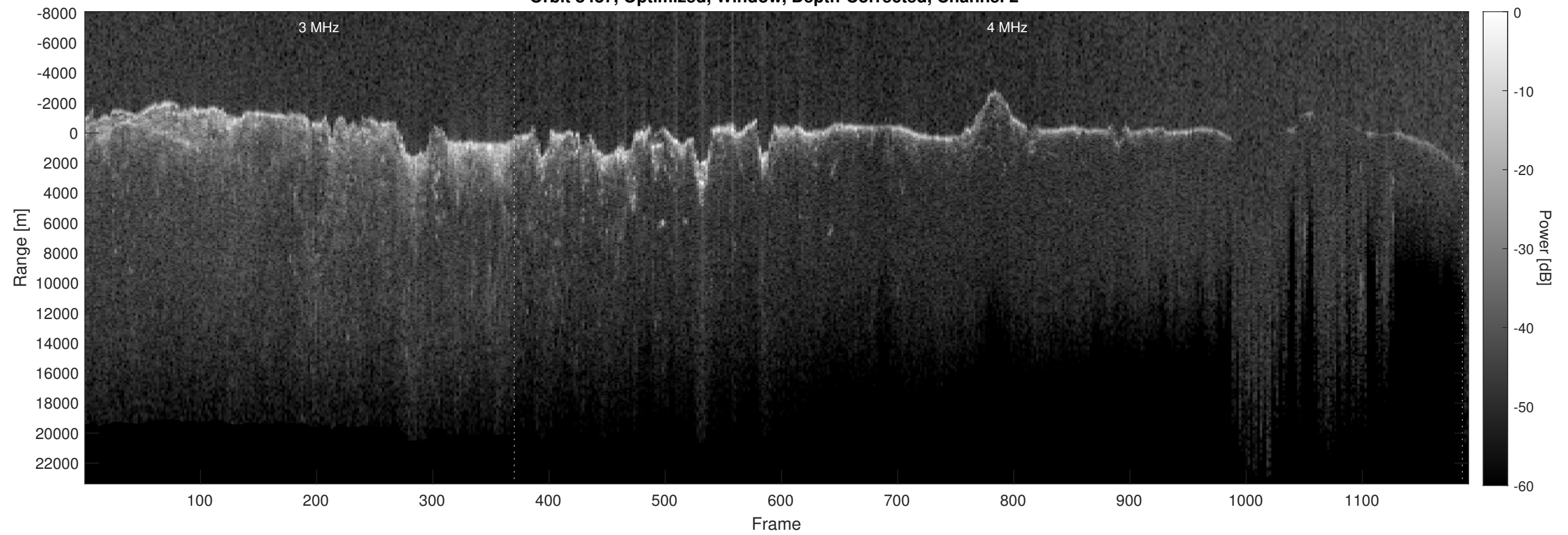
Orbit 8487, Optimized, Window, Depth-Corrected, Channel 2
