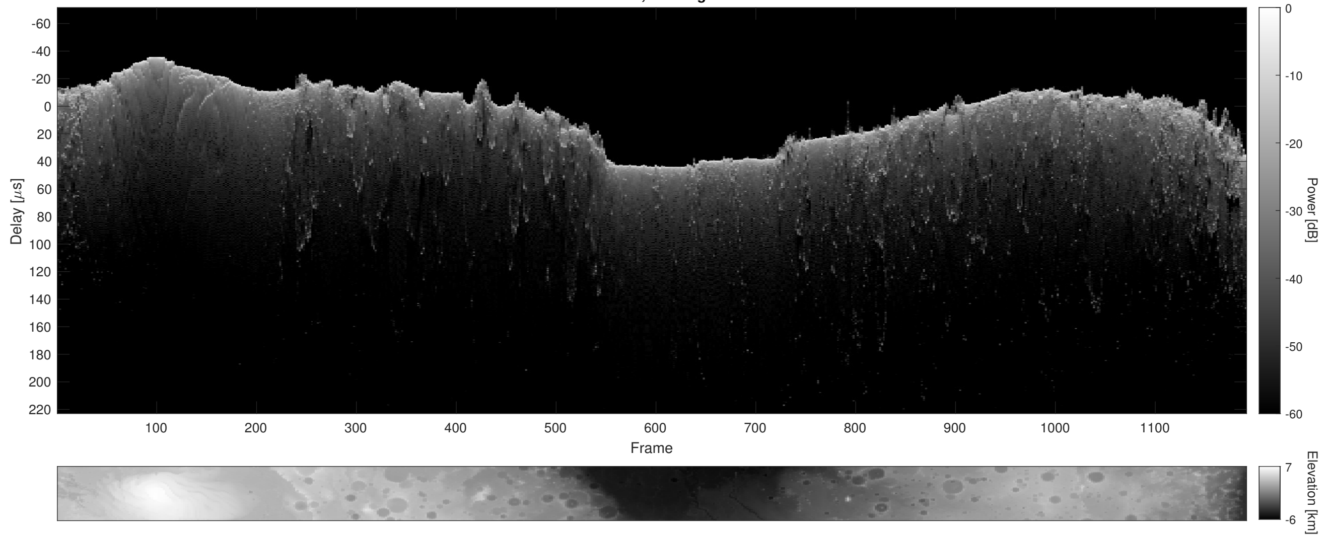
Orbit 8489, Cluttergram
