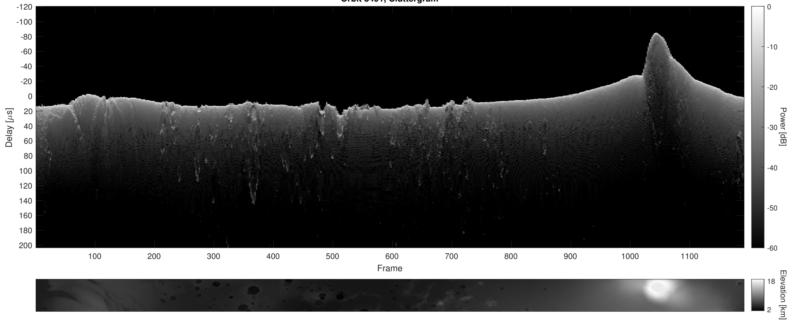
Orbit 8491, Cluttergram
