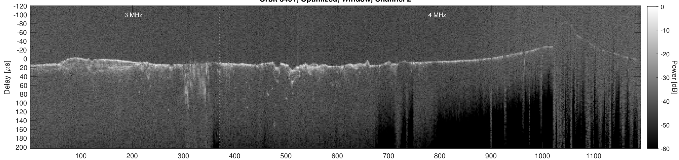
Orbit 8491, Cluttergram
