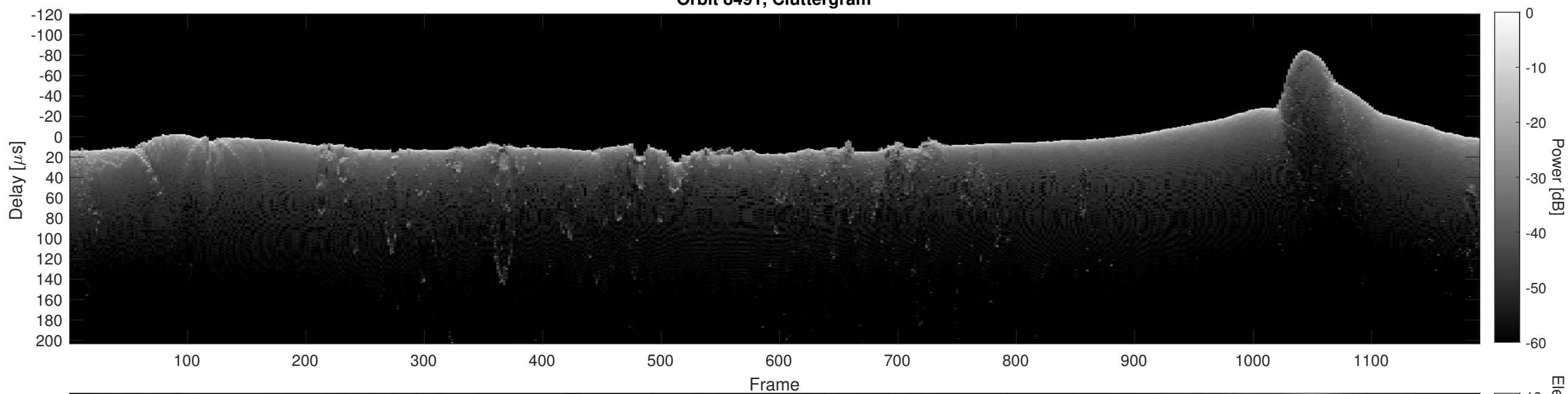
Orbit 8491, Cluttergram
