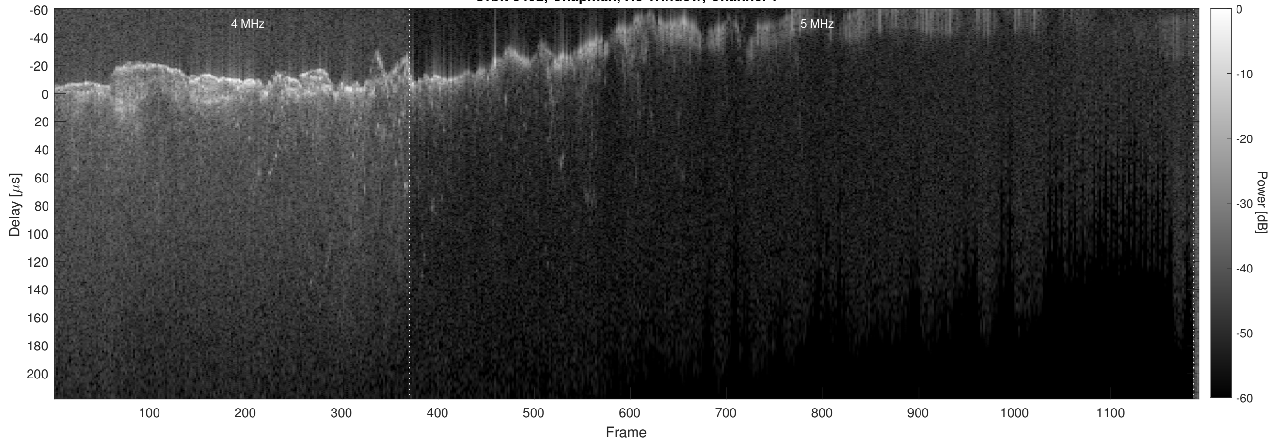
Orbit 8492, Chapman, No Window, Channel 2
