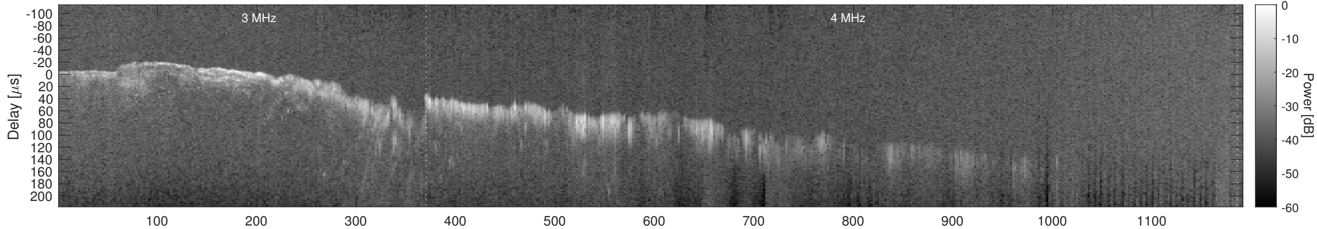
Orbit 8492, Window, Channel 2, Chapman
