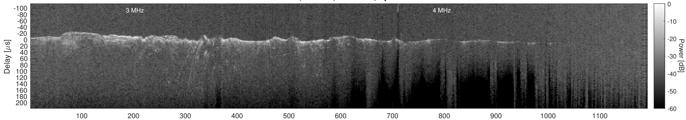
Orbit 8492, Cluttergram
