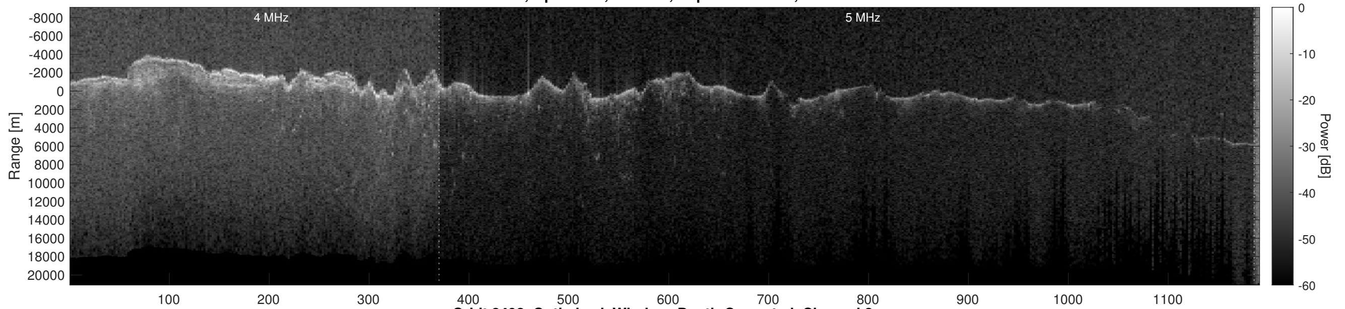
Orbit 8492, Optimized, Window, Depth-Corrected, Channel 2
