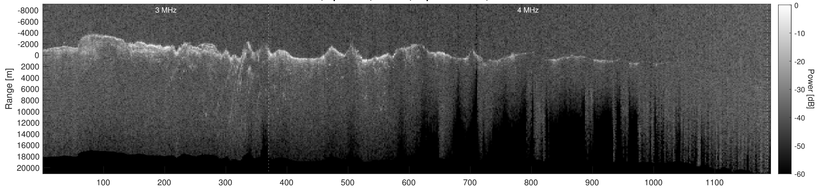
Orbit 8492, Depth-Corrected Cluttergram
