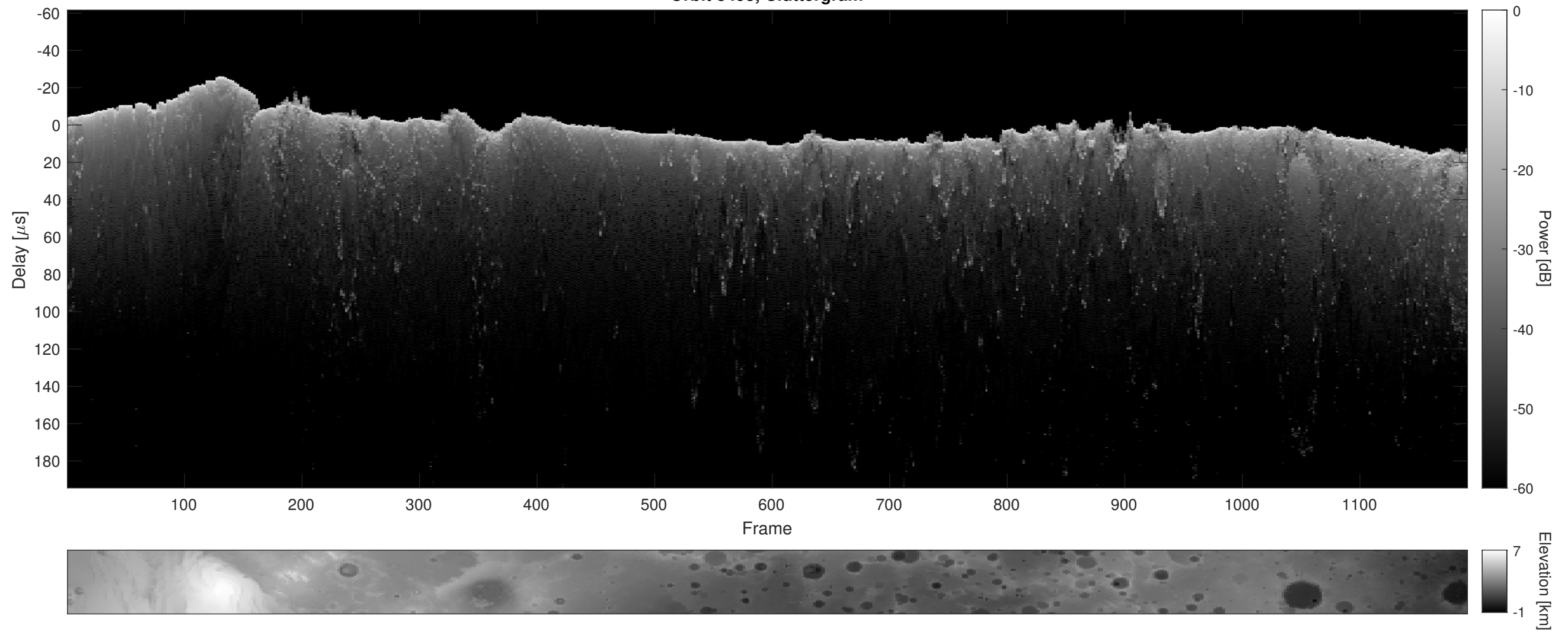
Orbit 8493, Cluttergram
